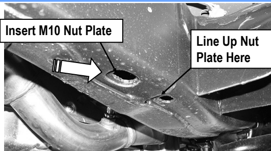
(Fig 3) Passenger Front Support Bracket Mounting Location
