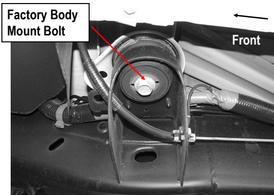
(Fig 1) Passenger Side Front Mounting Location Pictured
