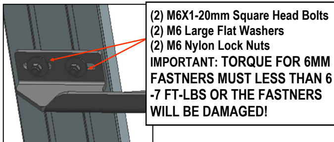
(Fig 15) Running Board Installed Onto Mounting Bracket
