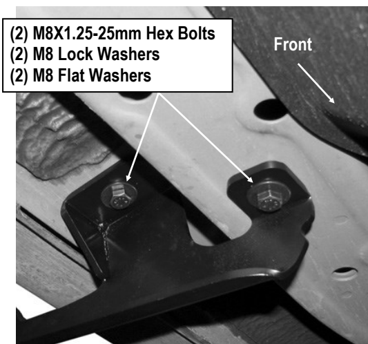
(Fig 7) Driver Side Center Mounting Bracket Installation
