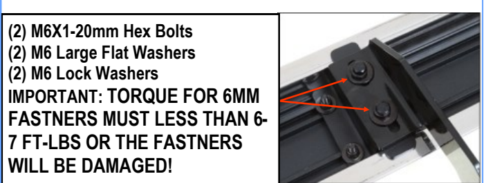
(Fig 17) Step Bar Installed on Bracket Installed (Example)
