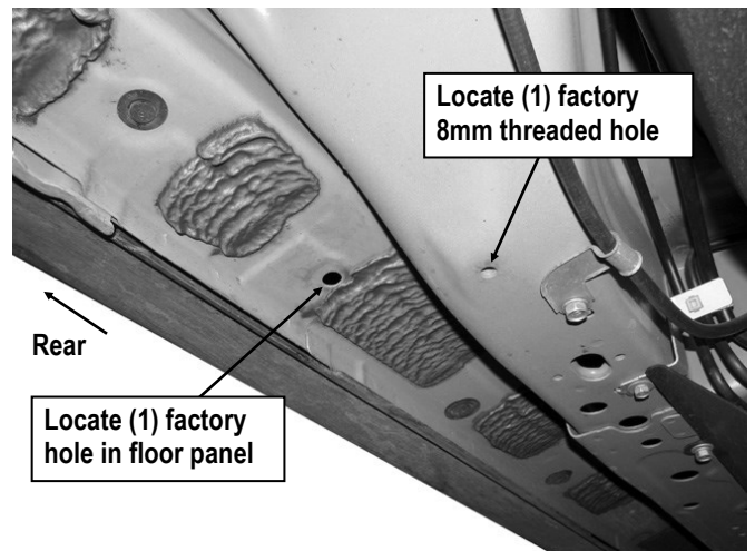
(Fig 8) Driver Side Rear Mounting Location Pictured
