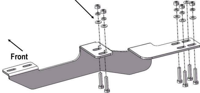
(Fig 2) Driver Front Mounting Bracket Installation
