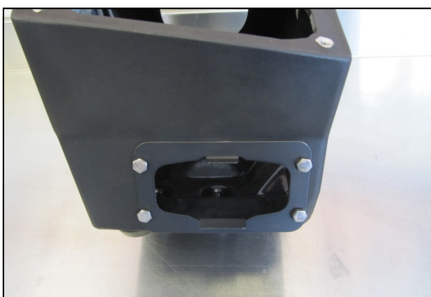
4. Install the Air Scoop Bracket (#4) into the Cold Air Box as shown by using four 1/4-20 x 5/8 Hex Bolts (#11), 1/4" Flat Washers (#12), and 1/4" Nylon Nuts (#13).
